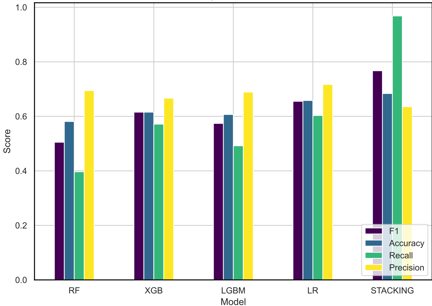
Model Comparison Performance
